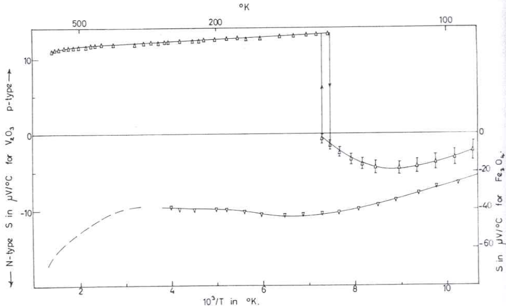
Figure 6.3: Thermopower in V_2O_3 ( \triangle , upper line) versus inverse temperature, left scale. The temperature gradient is perpendicular to the hexagonal c-axis. Right scale: Thermopower of Fe_3O_4 ( \nabla , lower line) [101].
