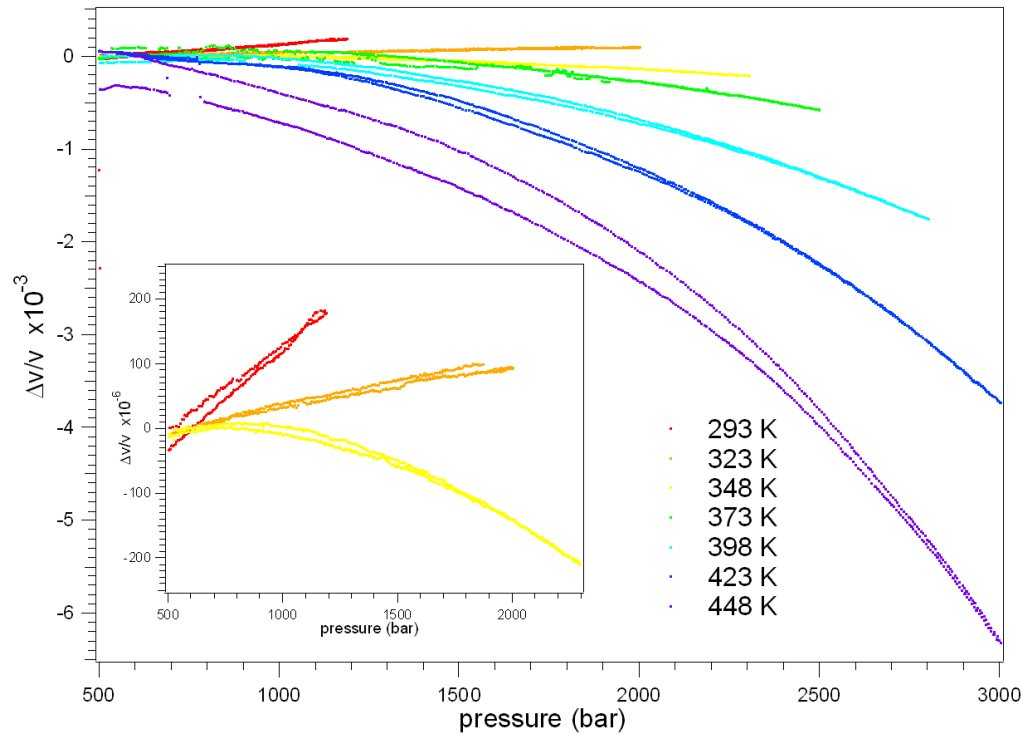
Figure 5.9: Pressure dependence of the relative sound speed for Cr doped V_2O_3 at different fixed temperatures below T_C in the pressure range of the insulating phase. Inset: zoom on the behaviour of the three lowest temperatures.
